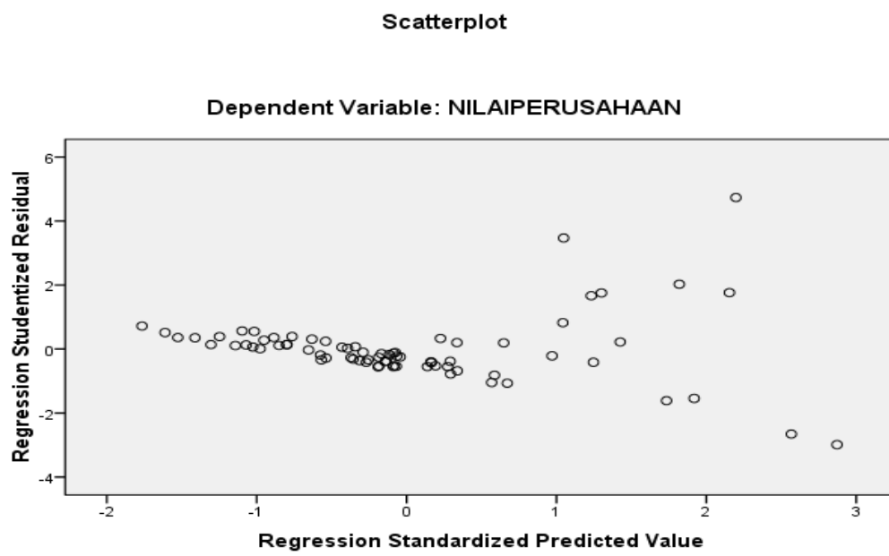
Gambar 4.4 Scatterplot
