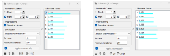
(a) Silhouette score data outlier K-Means 2021 (b) Silhouette score tanpa data outlier K-Means 2021
