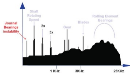
Gambar 5. Frequency Range (Pruftechnik, 2004)
