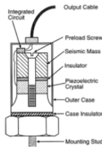
Gambar 2. Accelerometer (Vibrasi blog's, 2009)
