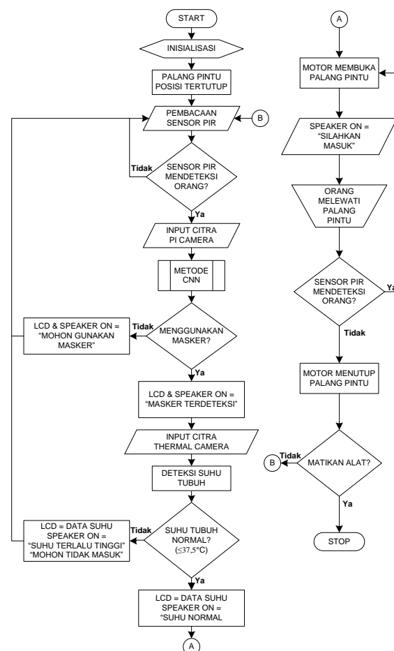
Gambar 2. Flowchart System
