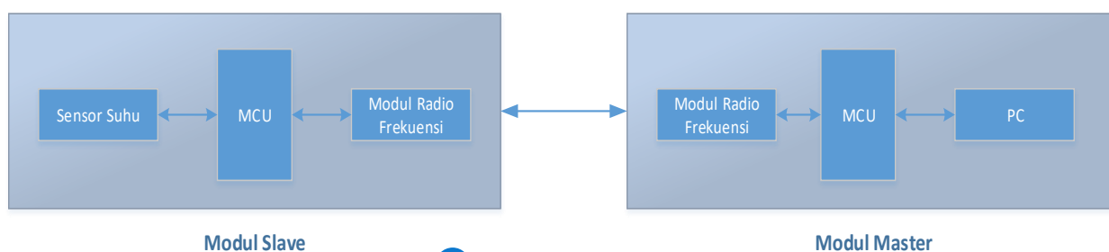
Gambar 2 Diagram Blok
