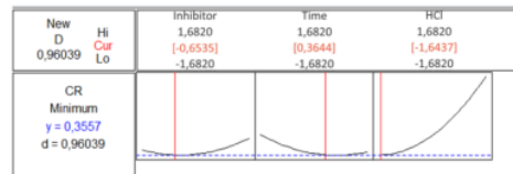
Figure 4. Response optimization.
