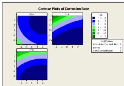
Figure 3. Contour plots of corrosion rate.
