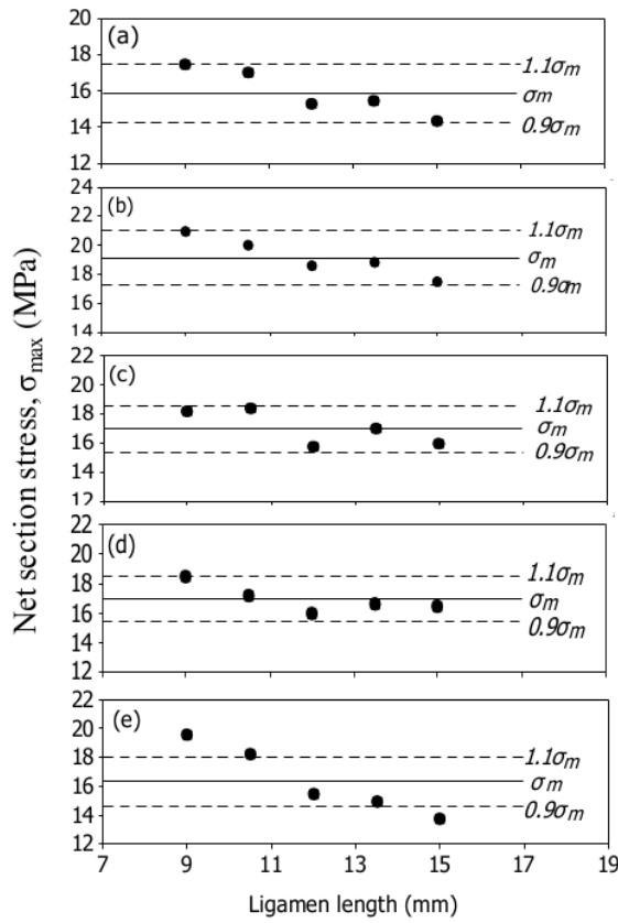
Fig. 5. Stress criteria according to ESIS protocol of EWF: (a) pure HDPE, (b) 5 wt.% zeolite/HDPPE, (c) 10 wt.% zeolite/HDPPE, (d) 15 wt.% zeolite/HDPPE, and (e) 20 wt.% zeolite/HDPPE.
