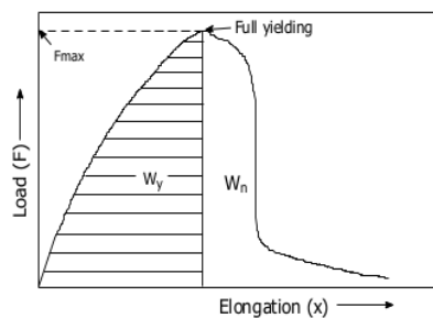
Fig. 2. Schematic explanation of energy partitioned EWF method [28].
