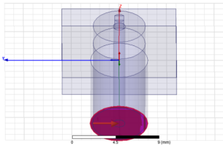
Gambar 3. Lumped Port
