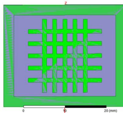
Gambar 5. Groundplane
