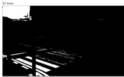
Gambar 5. pengujian threshold 200
