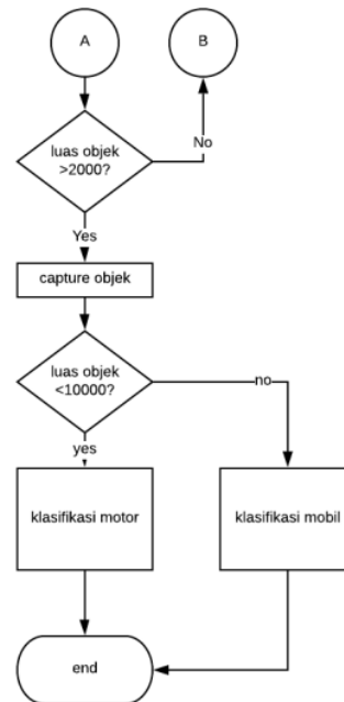
Gambar 2. Flowchart system
