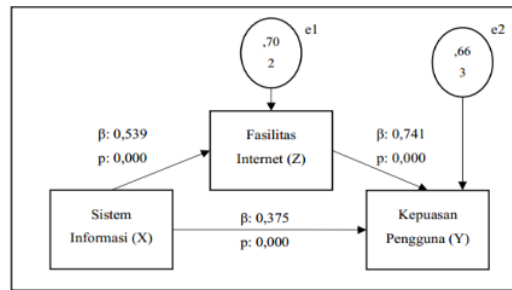
Figure 2:- Path Diagram Results
