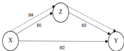
Figure 1:- Structural Equation Model Source: data processed (2022)
