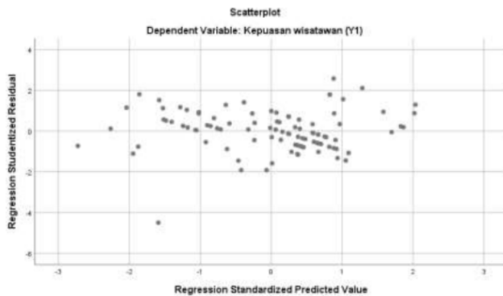
Figure 1: Heteroscedasticity Test Results Substructure Model 1
