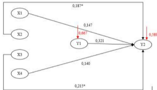
Figure 4: Pathway II Equation Model
