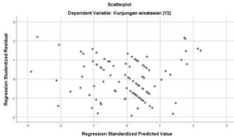
Figure 2: Heteroscedasticity Test Results Substructure Model 2
