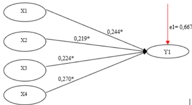
Figure 3: Pathway I Equation Model
