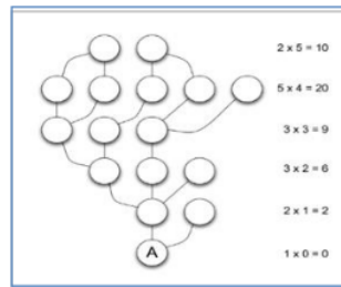
Figure 1. Justified graphs [13].
