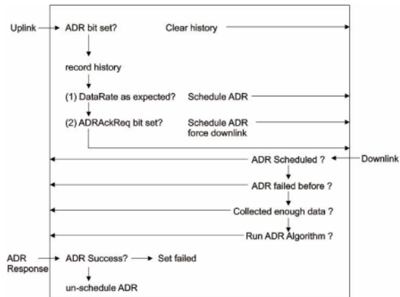
Fig. 3. Adaptive Data Rate Schedule Mechanism.
