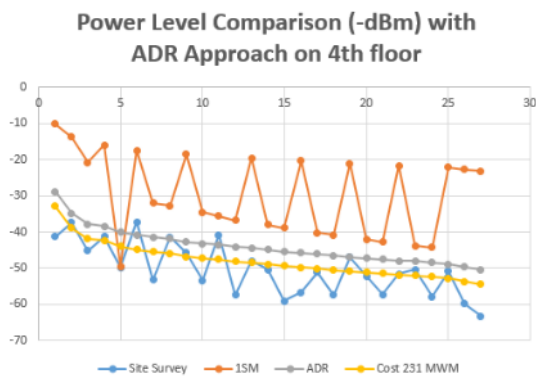
Fig. 8. Power Level Comparison on 4 th Floor.
