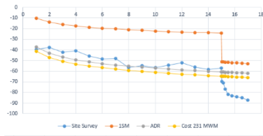
Fig. 6. Power Level Comparison on 2 nd Floor.
