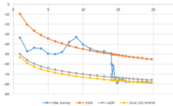
Fig. 5. Power Level Comparison on 1 st Floor.
