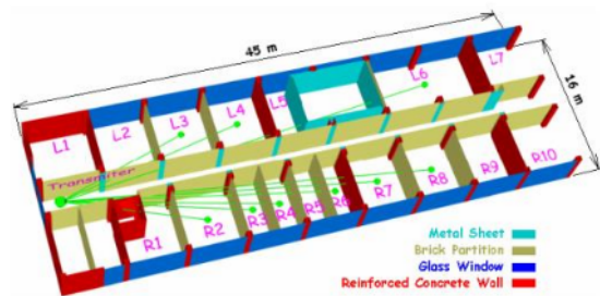
Fig. 1. Geometries Multi-Wall Model.
