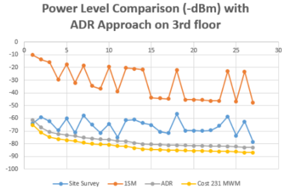
Fig. 7. Power Level Comparison on 3 rd Floor.
