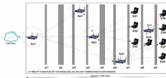
Fig. 2. Adaptive Data Rate Mechanism on Multi Wall.
