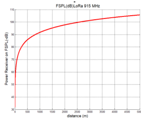
Fig. 24. Power Receiver of LoRa Module 915 MHz.
