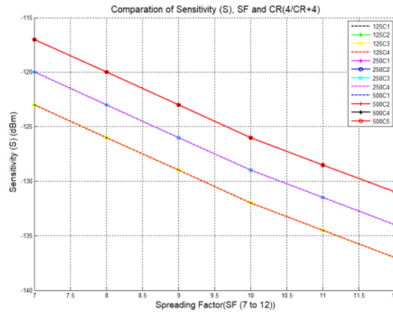
Fig. 9. Sensitivity of LoRa.
