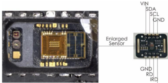
Fig. 2. Pulse Oximetry and Heart Rate Sensor Pins.
