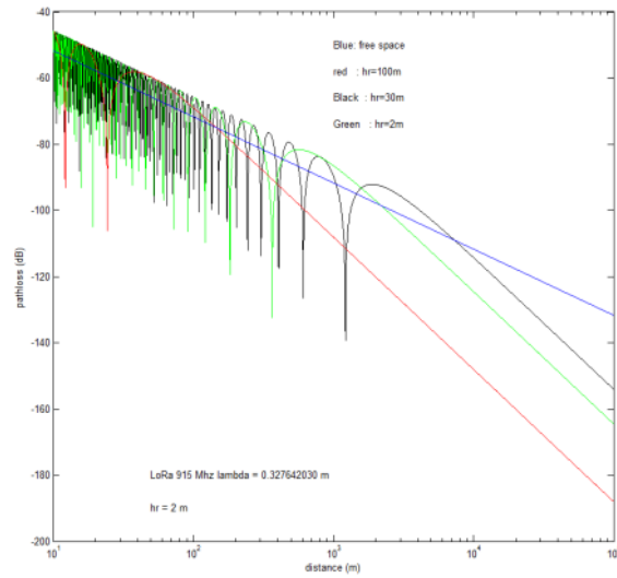
Fig. 14. LoRa 915 MHz Pathloss [dBm] of 2-Ray Ground Reflection Model.
