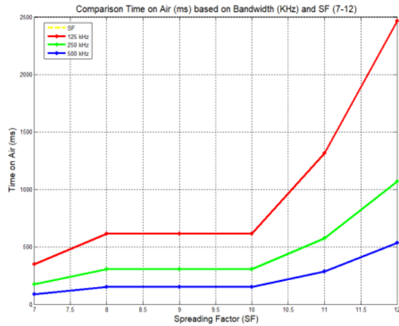
Fig. 12. ToA (ms) with SF.
