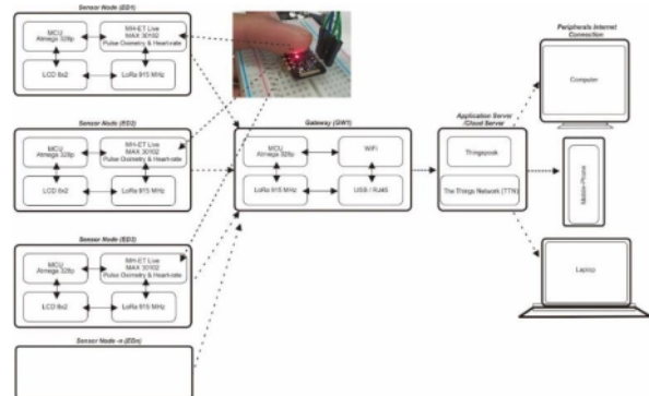
Fig. 8. Blog Diagram on this Research.
