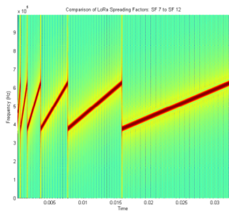
Fig. 5. Comparison Spreading Factor (SF) on 250 kHz Frequency.
