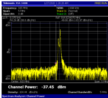
Fig. 27. LoRa Signal use a Signal Analyzer.
