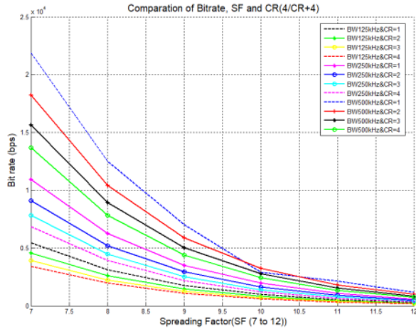
Fig. 11. Comparison of Bitrate (BW), SF and CR (4/CR+4).
