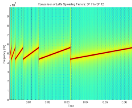
Fig. 4. Comparison Spreading Factor (SF) on 125 kHz Frequency.
