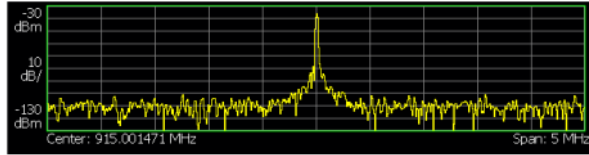
Fig. 25. LoRa Signal Analyze with Tectronix RSA 3408B Analyzer.
