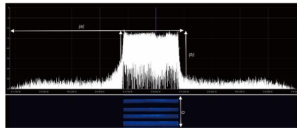
Fig. 24. LoRa Signal Analyze with SDR v.1.0.0.1700 RTL-SDR.
