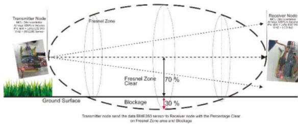
Fig. 14. Fresnel Zone 70% Clear.
