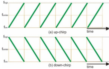
Fig. 4. Up and Down-Chirp Signal LoRa.
