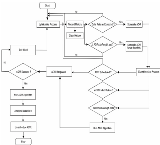
Fig. 19. Adaptive Data Rate (ADR) Flowchart.
