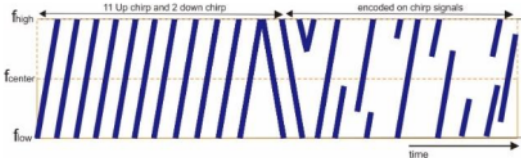
Fig. 5. LoRa Signal with Encoded (data) on.
