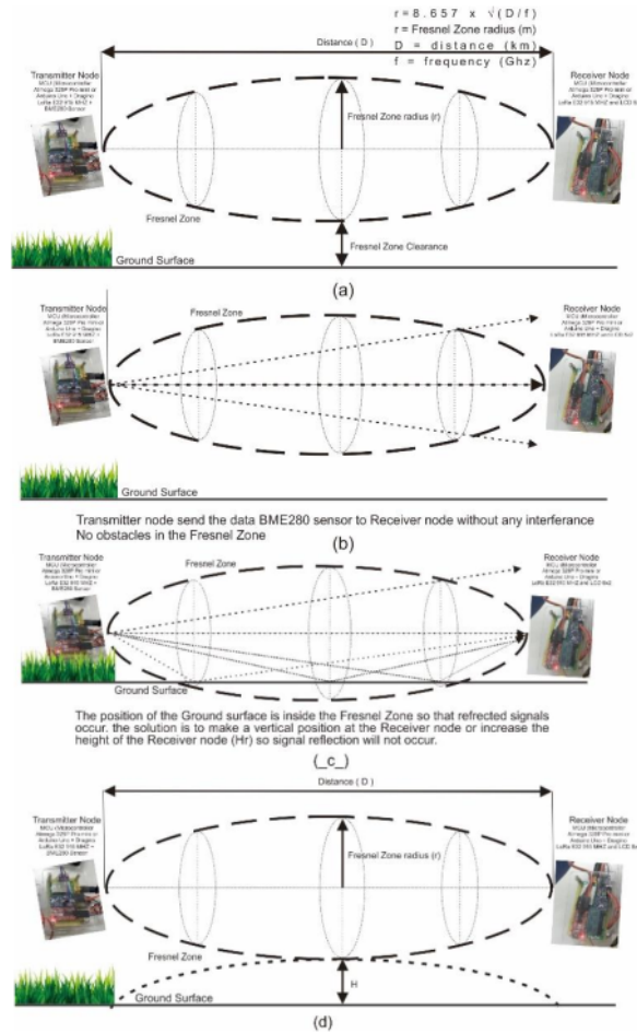
Fig. 13. Conditions of Fresnel Zone Theory.
