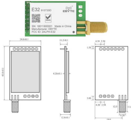
Fig. 11. LoRa E32 915T20D and Dimension.
