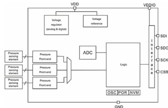
Fig. 6. Block Diagram of BME280 Sensor.
