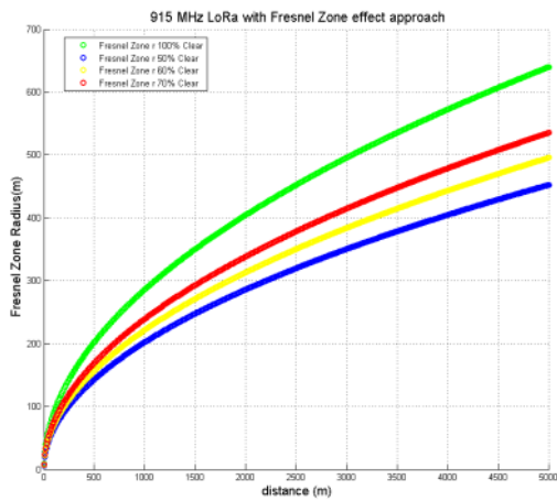
Fig. 15. Comparison of Fresnel Zone Clear Percentage (%).
