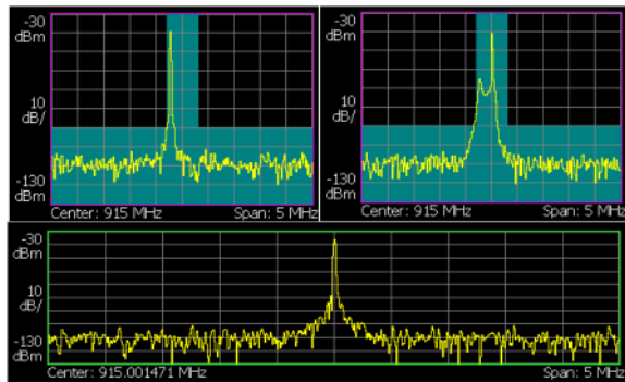
Fig. 27. Transmit Power LoRa Signal (dB).
