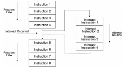
Fig. 20. Interrupt Process.
