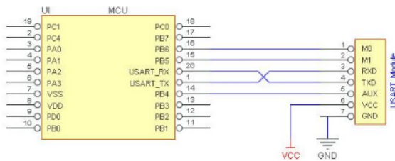
Fig. 12. Circuit Diagram of LoRa E32 915T20D.
