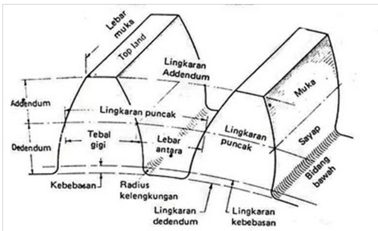
Gambar 2.4 Involut gear .
