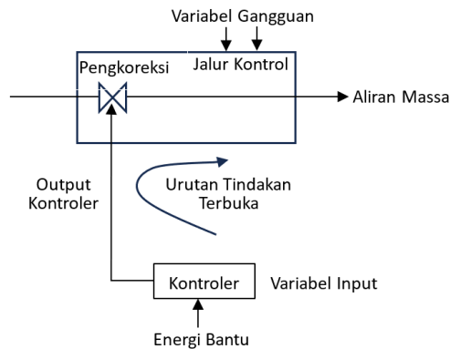
Gambar 1.6 Diagram istem kontrol open-loop .
