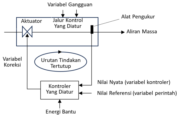
Gambar 1.8 Sistem kontrol closed-loop .
