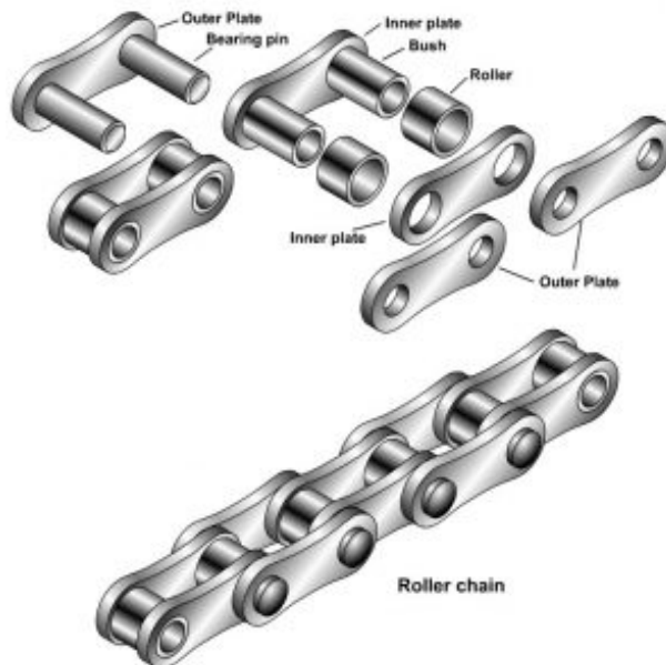
Gambar 2.19 Rantai roller .
