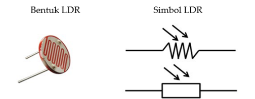
Gambar 4.11 Light Dependent Resistor - LDR
