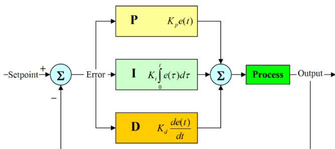
Gambar 5.3 Ilustrasi diagram blok sistem kontrol Proporsional-Integral-Derivatif .
