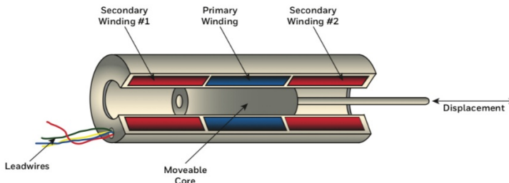
Gambar 4.8 Sensor LVDT ( linear variable differential transformer ).
