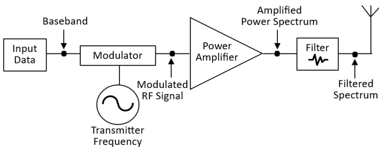
Gambar 1.5 Diagram blok sistem pemancar RF (Radio Frequency Transmitter System).
