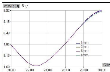
Figure 4.7 Comparison VSWR L_s variation
