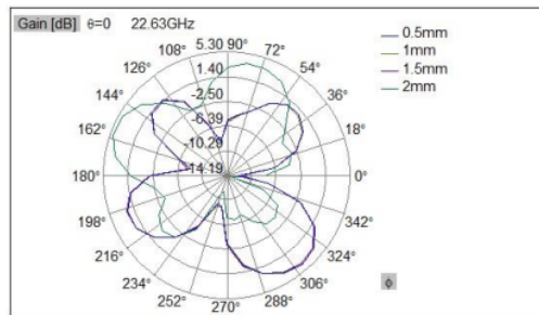
Figure 4.3. affected Gain by W_s variation
