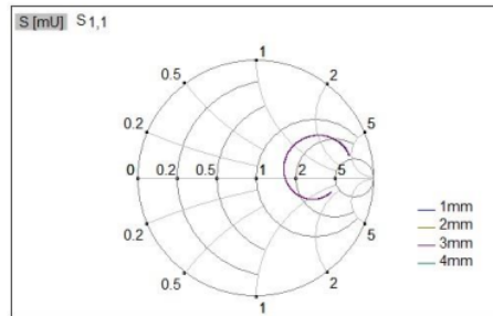
Figure 4.4 Smith Chart affected by L_s variation
