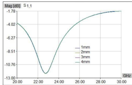
Figure 4.1. S11 affected by L_s variation
