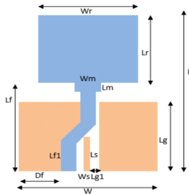
Figure 3.1. Design antenna planar monopole
