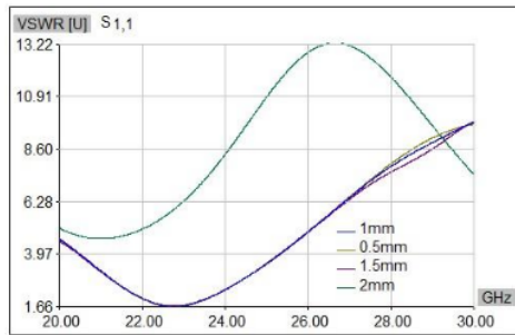
Figure 4.6 Comparison VSWR W_s variation
