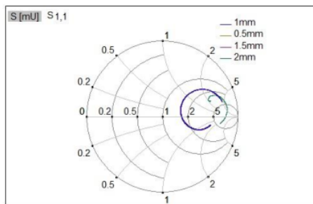
Figure 4.5 Smith Chart affected by W_s variation
