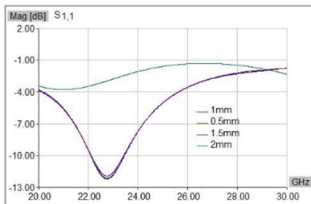
Figure 4.2. S11 affected by W_s variation
