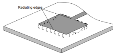
Figure 2.1 microstrip antenna
