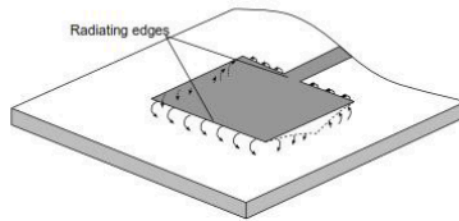
Figure 2.1 microstrip antenna
