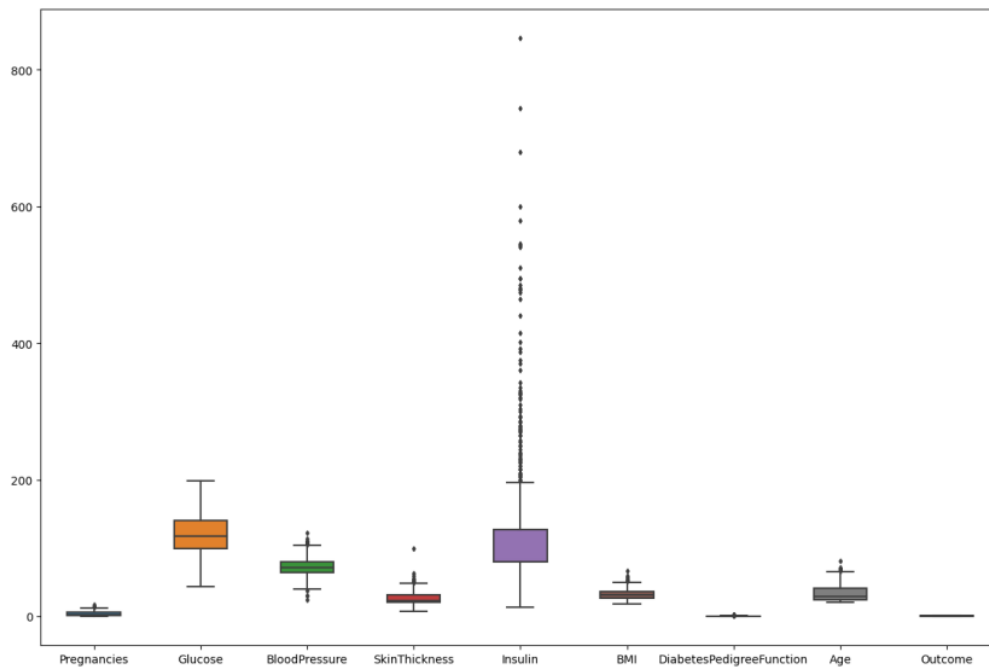
Gambar.2 Boxplot data analyst
