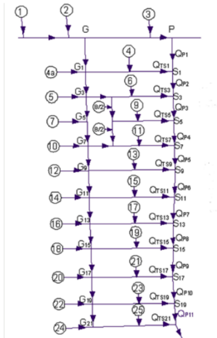
Figure 2. Road system at the study area
