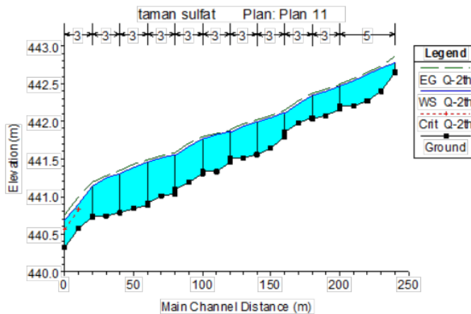
Figure 4. Long section of the main road
