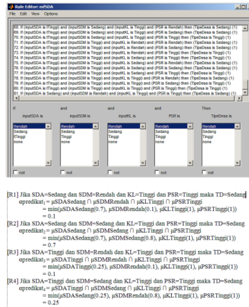
Gambar 8. Rule Editor
