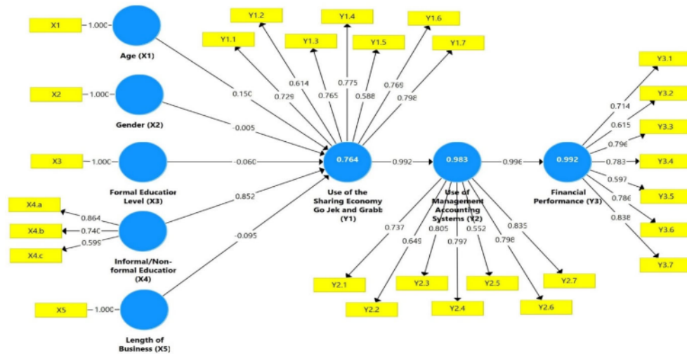
Fig. 3. PLS Algorithm
