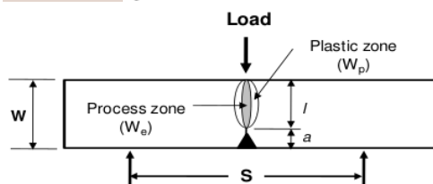
Figure 1. SENB specimen geometry for the EWF method
