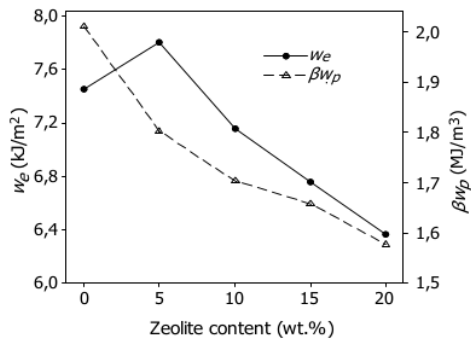
Figure 3. The w_e and w_f as function of zeolite content
