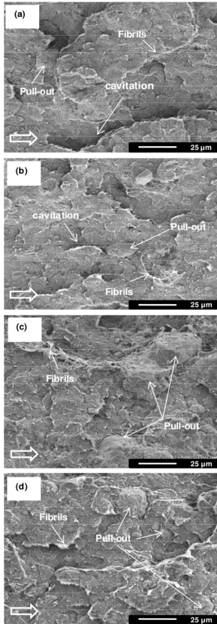
Figure 8. The SEM micrograph of the fracture surface taken on middle of ligament length; (a) 15 wt.% zeolite/HDPPE, (b) 10 wt.% zeolite/HDPPE, (c) 15 wt.% zeolite/HDPPE, and (d) 20 wt.% zeolite/HDPPE
