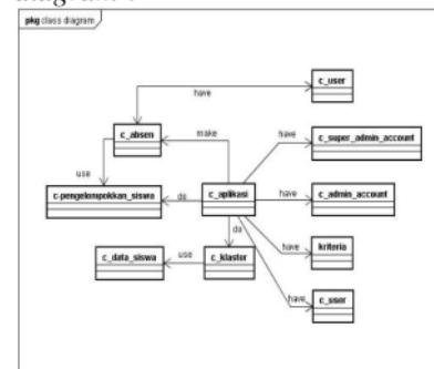
Gambar 5. Class Diagram
