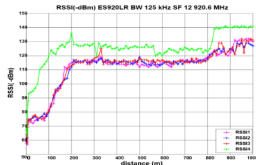
Fig. 6. The experimental data multi node on LoS and Non-LOS.
