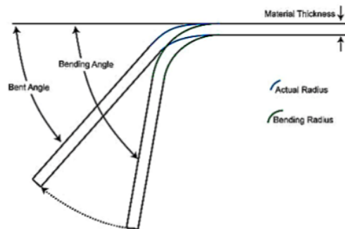
Gambar 1. Springback Effect [1]
