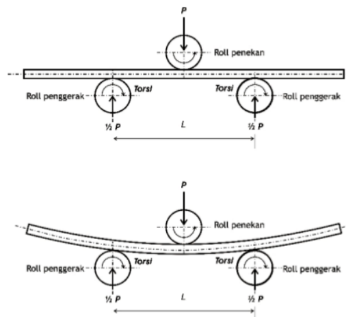
Gambar 6. Proses Roll Bending Pipa
