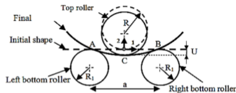
Gambar 2. Mekanisme Proses Roll Bending [2]
