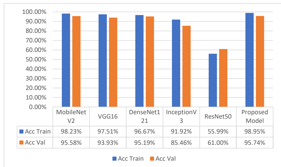
Figure 6. Performance Comparison with Other CNN Models.
